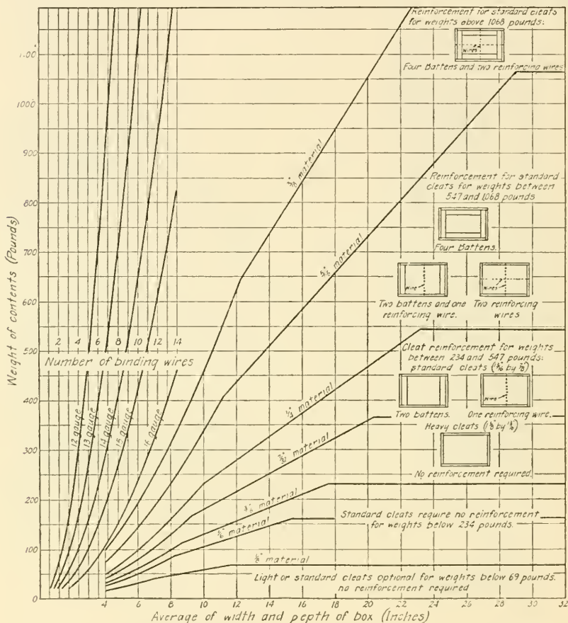
FIGURE 33.—Minimum thicknesses of sheet material and number and size of binding wires for wire-bound boxes made of Group 4 woods
